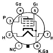
BOTTOM VIEW BASING DIAGRAM JEDEC 7AC
